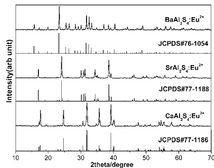
Figure 1. XRD patterns of MAI 2 S 4 :Eu 2+ (M = Ca, Sr, and Ba).
