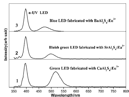
Figure 3. The electroluminescence spectra of the fabricated PC-LEDs combined with CAS (1), SAS (2), and BAS (3) phosphors under 20-mA forward-bias current.
