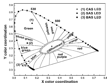
Figure 4. The CIE coordinates of PC-LEDs based on CAS (1), SAS (2), and BAS (3) under 20-mA forward-bias current in the CIE 1931 chromaticity diagram.
