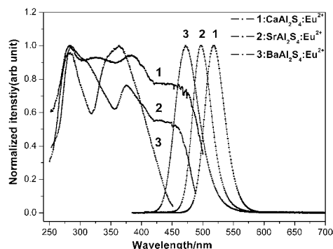
Figure 2. The normalized emission and excitation spectra of the thioaluminate phosphors CAS (1), SAS (2), and BAS (3) at room temperature ( \lambda_{\text{ex}} = 395 nm, \lambda_{\text{em}} = 516 , 496, and 470 nm, respectively).
